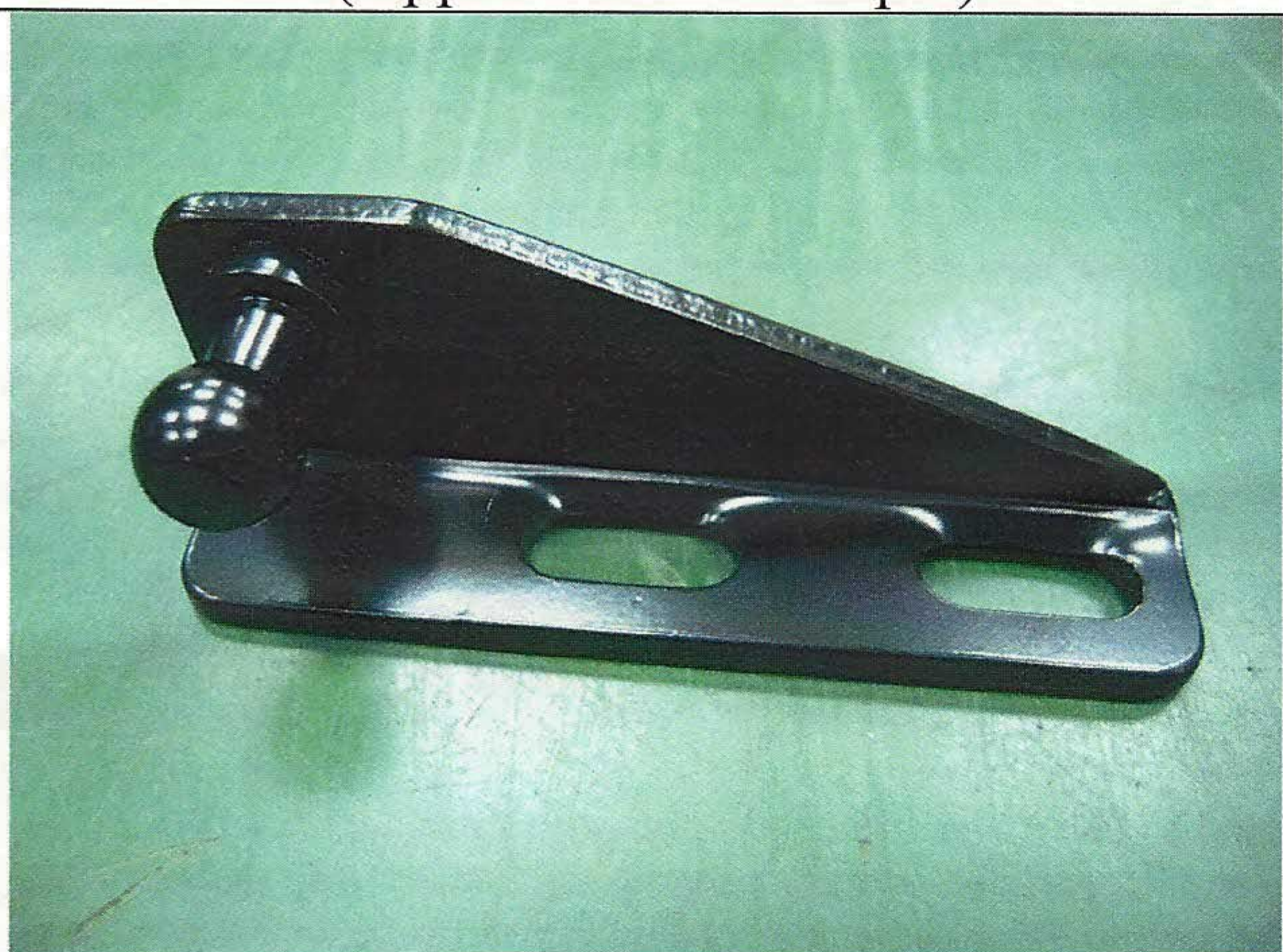
Photo "P" (Appearance of sample) BKT-26-L
