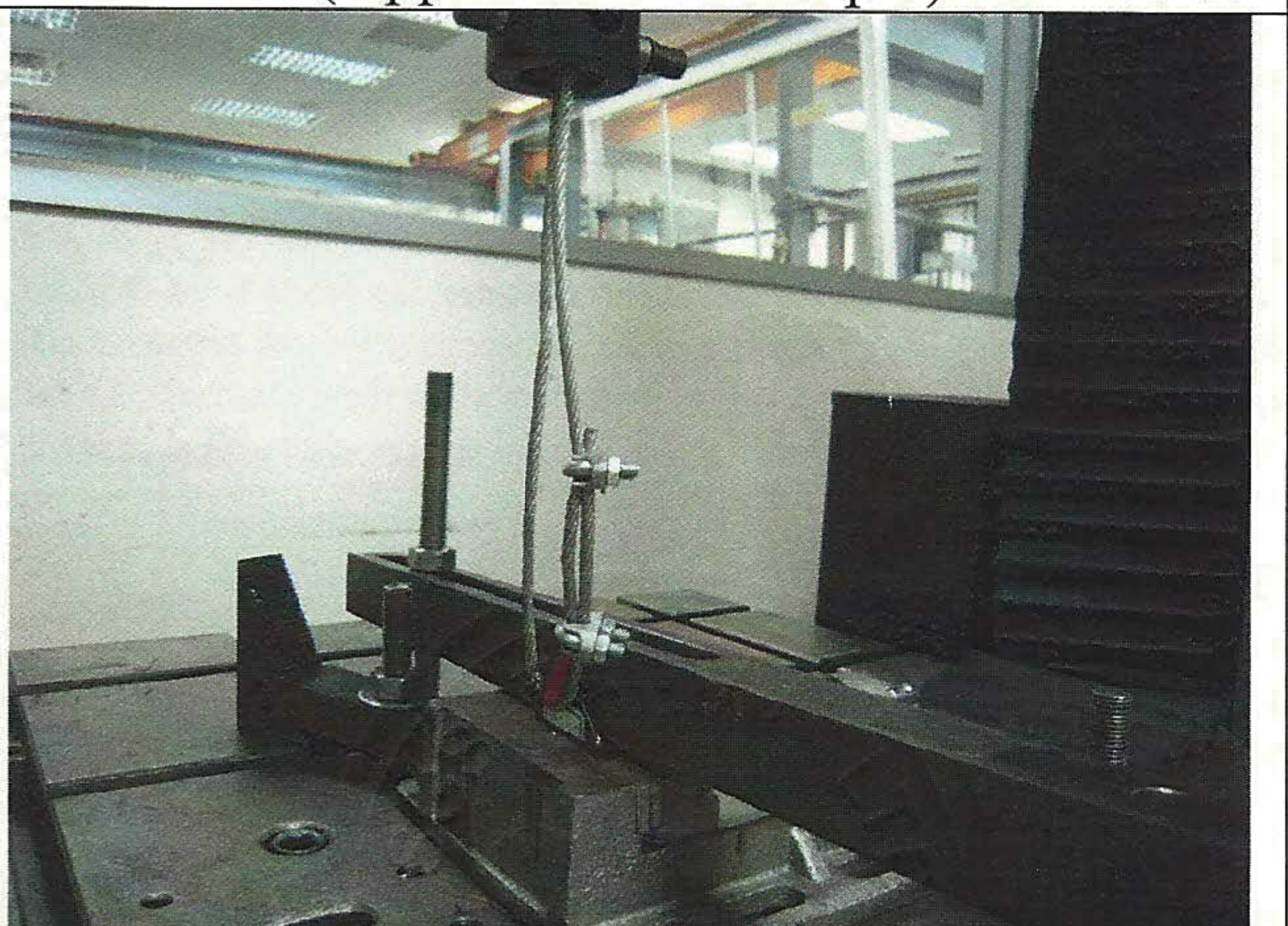
Photo "X" (Test setup)
